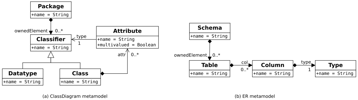
Fig. 2. Class diagram and ER metamodels.
