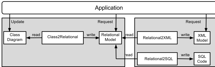
Fig. 1. The transformation chain: Class2Relational + Others.
