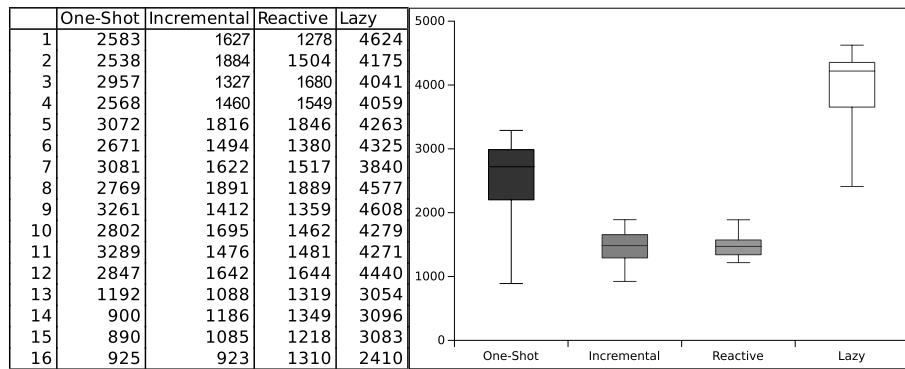
Fig. 8. Update & Read total time.
