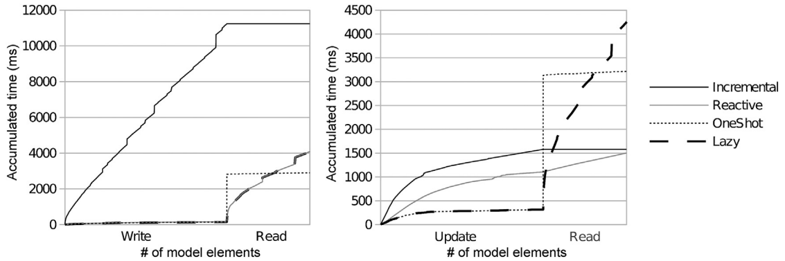
Fig. 6. Performance comparison for source model 1.
