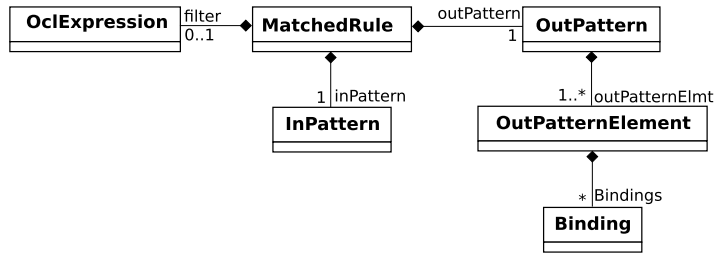
Fig. 5. ATL metamodel excerpt.
