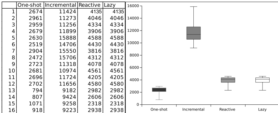
Fig. 7. Write &amp; Read total time.
