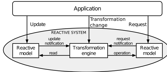
Fig. 4. Reactive transformation system.
