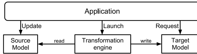
Fig. 3. Common model-driven application architecture.
